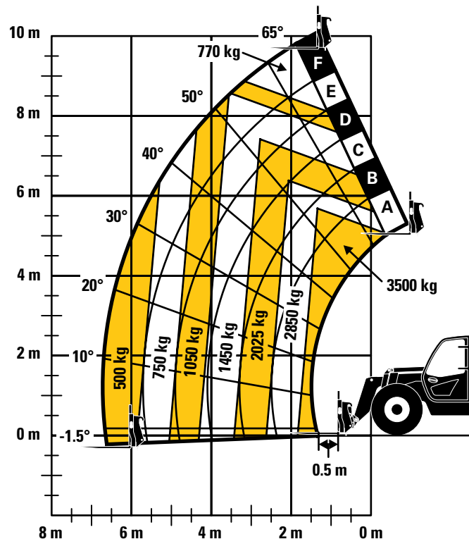
Ag Handler TH3510D
